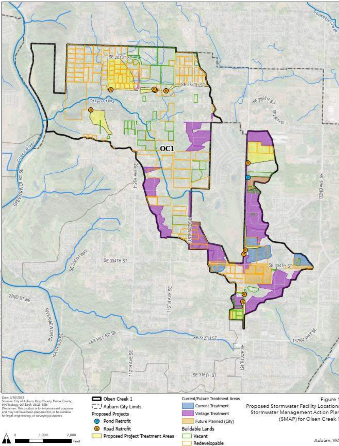
Figure 3. Proposed Stormwater Facility Retrofit Locations
